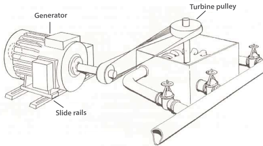
Figure 19 Quarter turn belt drive Source: Practical Action
