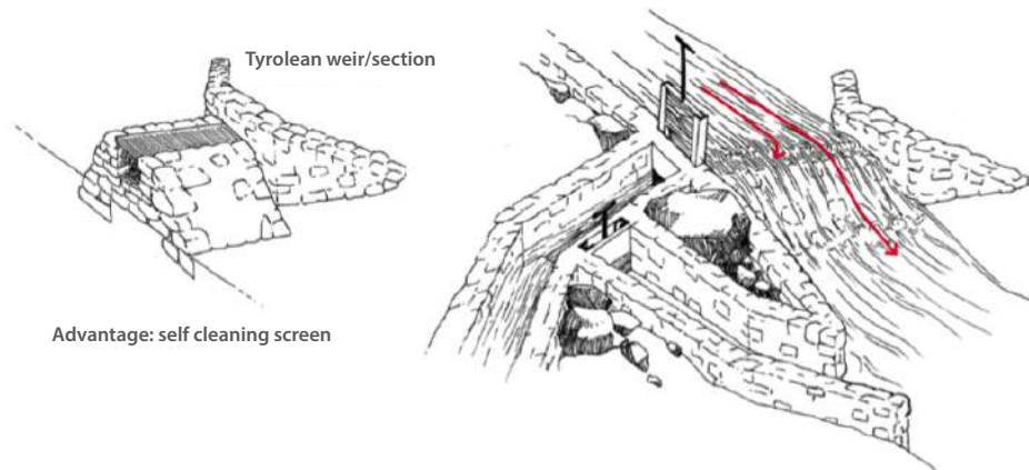
Figure 2: Tyrolean Weir construction 1 Source: Practical Action
