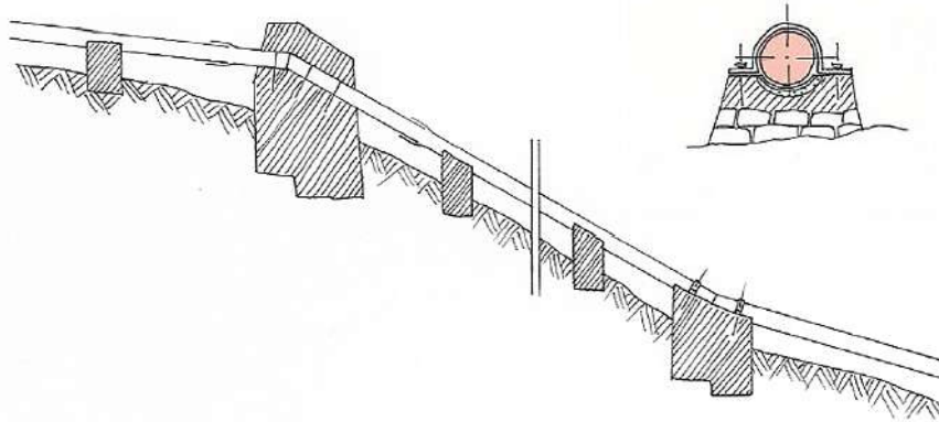
Figure 7 Penstock anchoring Source: Practical Action
